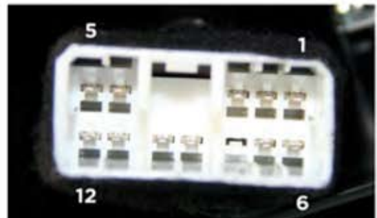
View of the connector in car
